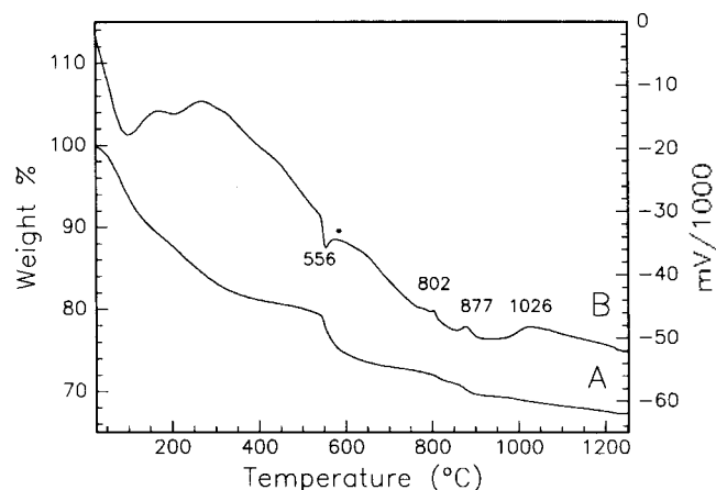
Figure 7. TG trace (A), and DTA curve (B) of vanadium-doped forsterite xerogel. The xerogel was heated in dry oxygen (200 mL/min) at a rate of 10°C/min.
