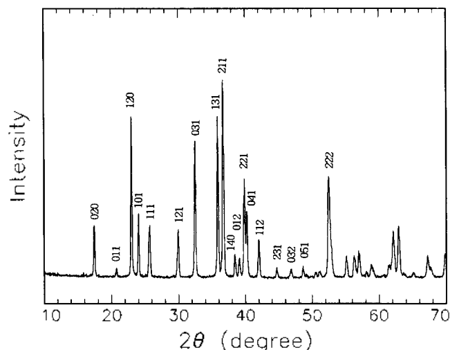
Figure 6. PXRD pattern taken from the polycrystalline powder of vanadium-doped forsterite obtained by heating the xerogel at 1100 °C in air.
