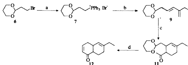
Scheme 1. (a) \text{PPh}_3 /toluene, reflux, (b) n -BuLi/THF, acrolein ( 8 ), (c) methyl vinyl ketone ( 10 ) in seal tube, 150 °C, (d) 3 N \text{HClO}_4 .
