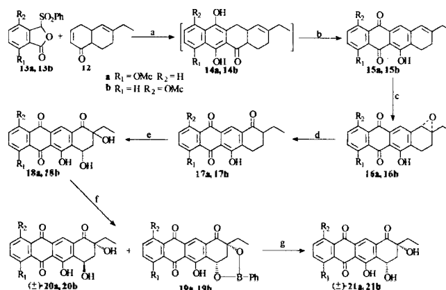
Scheme 2. (a) t -BuOLi/THF, -78 °C, rt, reflux, (b) \text{O}_2 /DMF, (c) m -CPBA/ \text{CH}_2\text{Cl}_2 , rt, 5 hr., (d) HF/Pyr (7:3)/THF, 0 °C (5 min), rt (8 hr), (e) t -BuOK, \text{P}(\text{OMe})_3 , \text{O}_2 /DMF, -15 °C, (f) PhB(OH) 2 , p -TsOH/toluene, (g) 2-methyl-2,4-pentanediol, AcOH/ \text{CH}_2\text{Cl}_2 /acetone.
