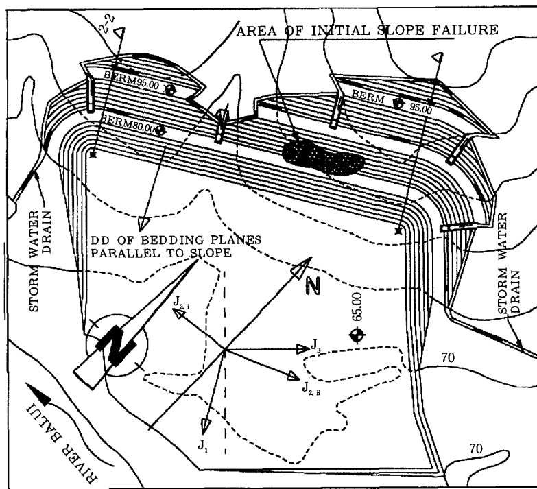
Figure 4. The locations of the local investigated slopes of the Inlet Area
