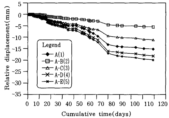
Figure 8. Results of monitoring measurements of Inlet slope section 3-3 after failure
