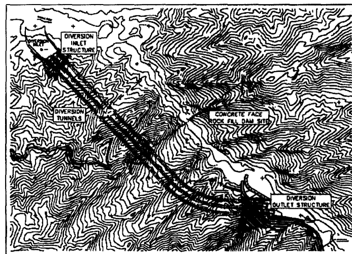
Figure1. Layout of the Bakun River Diversion Tunnelling Works
