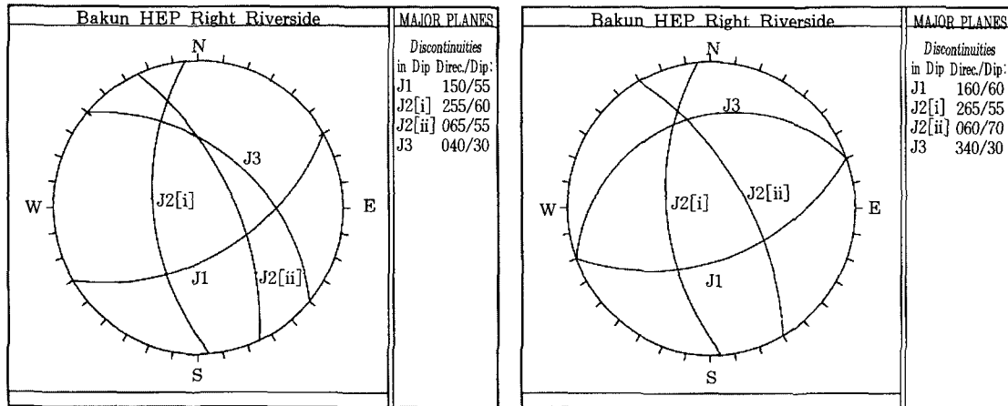
Figure 2. Discontinuities of Bakun Site(Jee, 1997)
