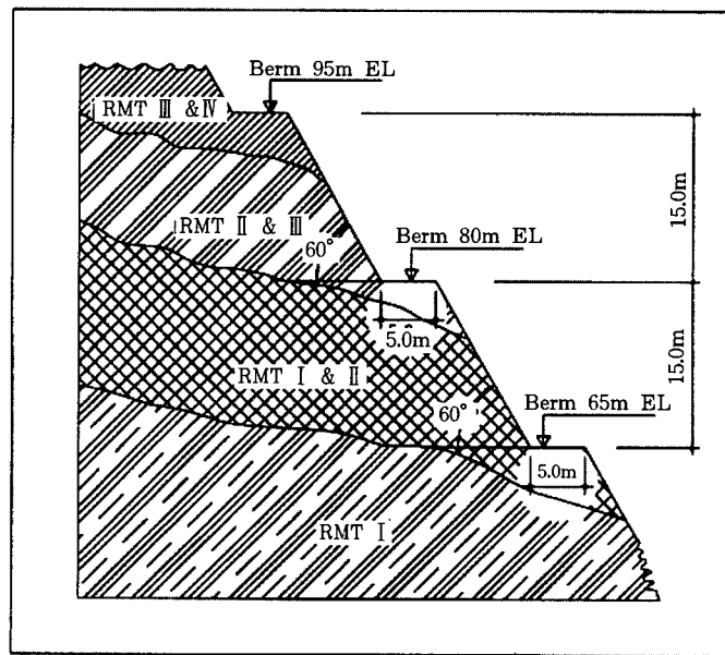
Figure 3. Typical geometry of the planned rock slopes(Jee, 1997)
