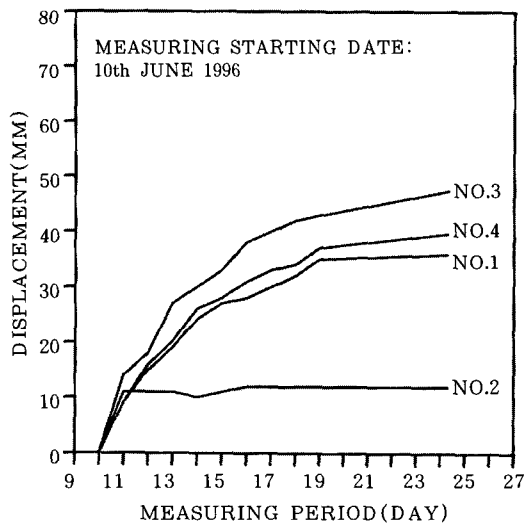
Figure 7. Results of monitoring measurements of Inlet slope section 3-3 before failure
