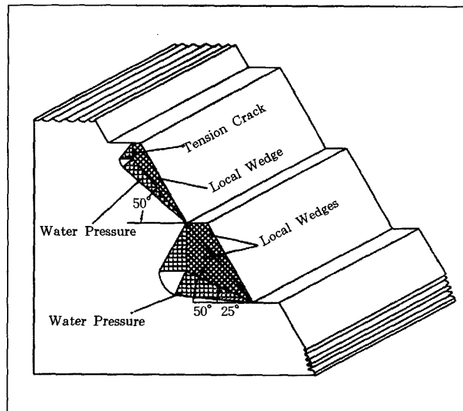
Figure 5. Plane wedge stability for local wedges
