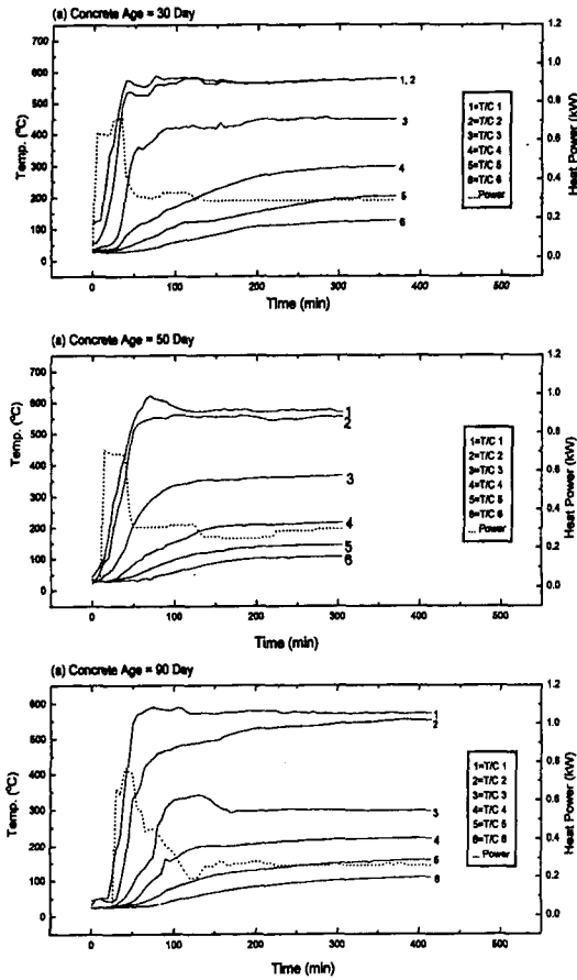
Fig. 6. Temperature Change of Test Article Assembly for Different Concrete Aging Temp. - Exp. Conditions: Sodium Mass = 250g, Heating Temp. = 550°C
