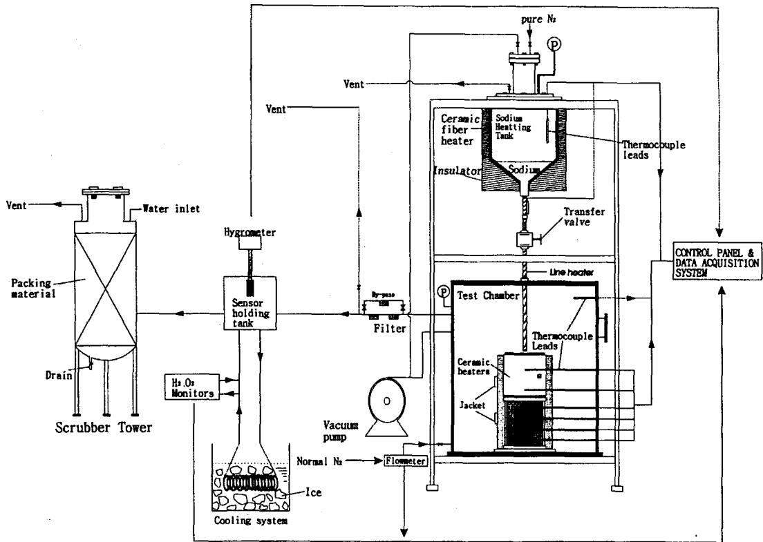
Fig. 1. Sodium-Concrete Reaction Test Facility
