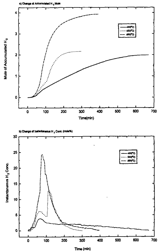
Fig. 5. Change of the Amount of H 2 Generated for Different Sodium Reservoir Heating Temp. - Exp. Conditions: Concrete Age = 45 Day, Sodium Mass = 250g
