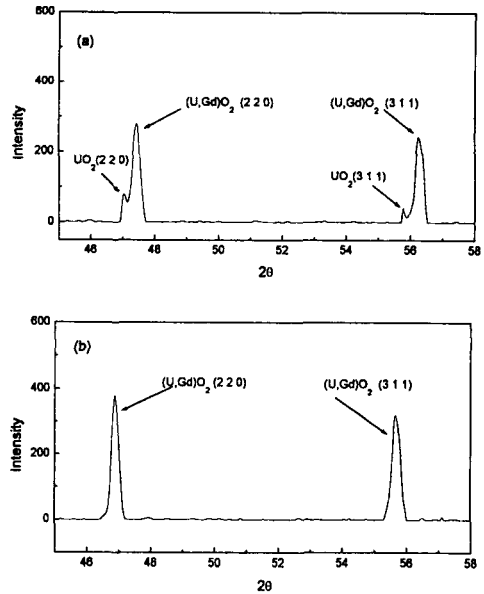
Fig. 13. X-ray Diffraction Patterns of UO 2 -15wt% Gd 2 O 3 Pellets Sintered in (a) H 2 , (b) H 2 -30CO 2
