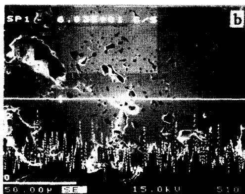
Fig. 11. Line Profile of Gd Concentration in Sintered \text{UO}_2 -10wt% \text{Gd}_2\text{O}_3 Pellets from Powder Type I (a) \text{H}_2 , (b) \text{H}_2 -30 \text{CO}_2
