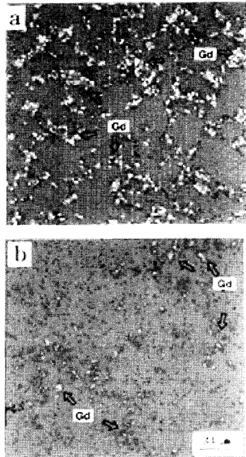
Fig. 4. Area Mapping of Gd Distribution in Green Pellets (a) powder type I, (b) powder type II
