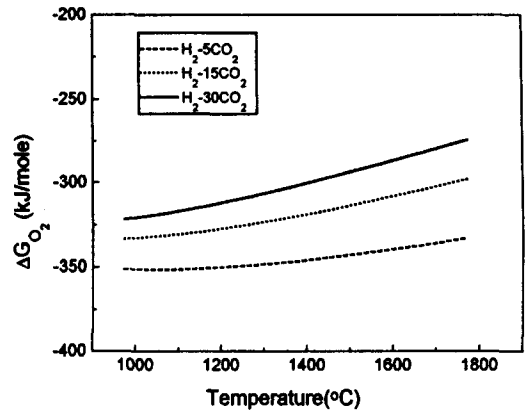
Fig. 2. Oxygen Potential of H 2 -CO 2 Mixed Gases
