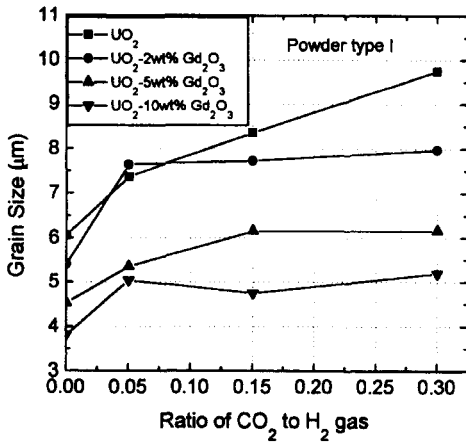
Fig. 12. Grain Sizes of UO 2 -Gd 2 O 3 Pellets of Powder Type I as a Function of Oxygen Potential
