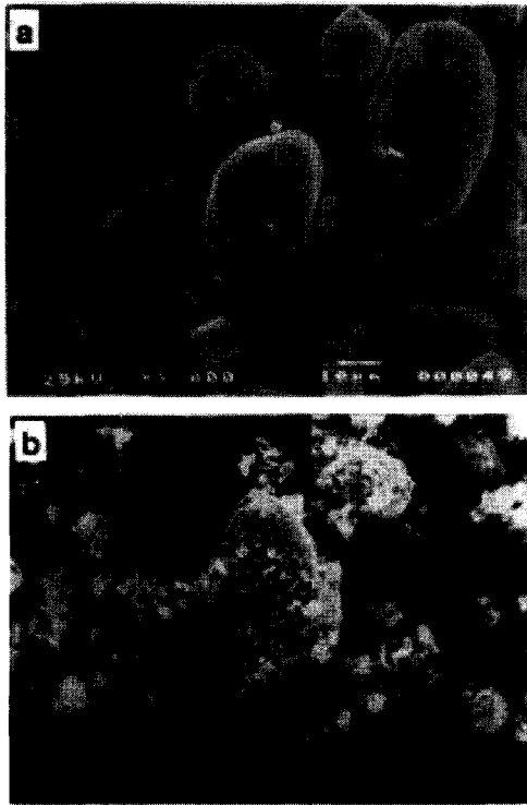
Fig. 3. SEM Micrographs of UO 2 Powders (a) AUC-UO 2 powder, (b) ADU-UO 2 powder
