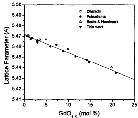
Fig. 14. Lattice Parameters of (U,Gd)O 2 Solid Solutions
