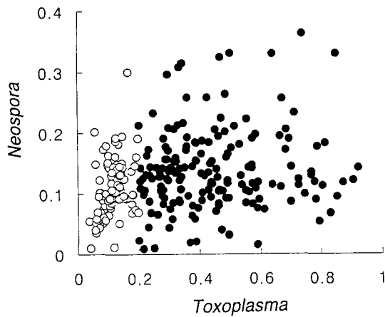
Fig. 1. Distribution of absorbance spots of Toxoplasma vs. Neospora . Closed circles indicate the Toxoplasma -positive group and open circles indicate the Toxoplasma -negative group.
