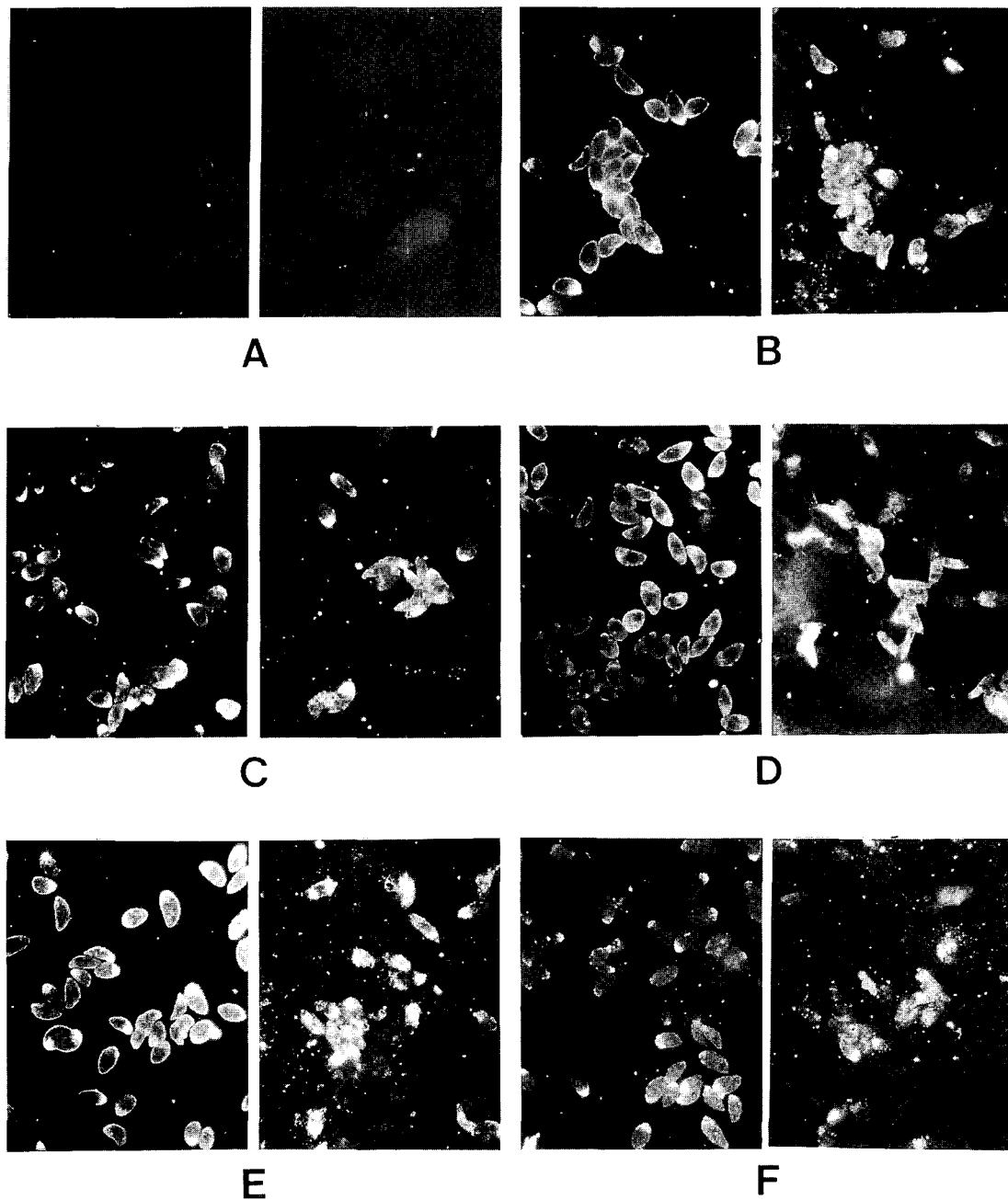
Fig. 3. Immunofluorescence photomicrographs of Toxoplasma gondii (left) and Neospora caninum (right). A , control with serum of lane 1 of the Toxoplasma -negative group; B , serum of lane 1; C , lane 4; D , lane 7; E , lane 10 of the Toxoplasma -positive group; F , lane 2 of the Toxoplasma -negative group, respectively.
