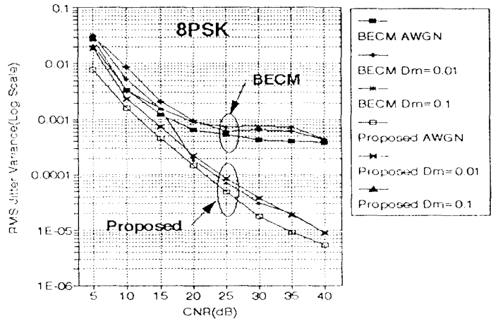
(a) 8PSK
