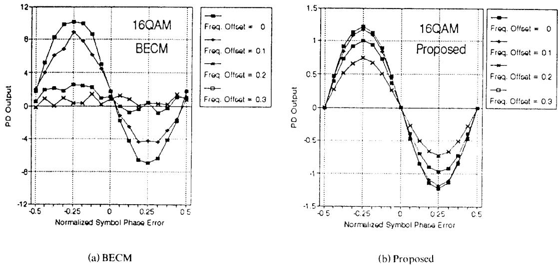
Fig. 5 PD Output versus Normalized Frequency Offset
