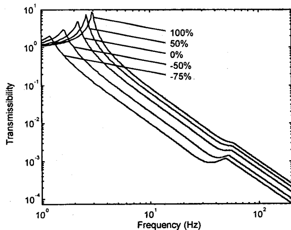
Fig. 9 Effect of rubber stiffness on controlled mount performance
