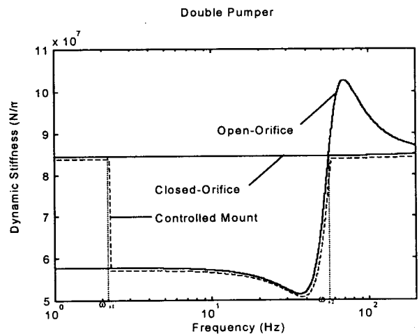
Fig. 7 Dynamic stiffness of fluid mount with open and closed orifice
