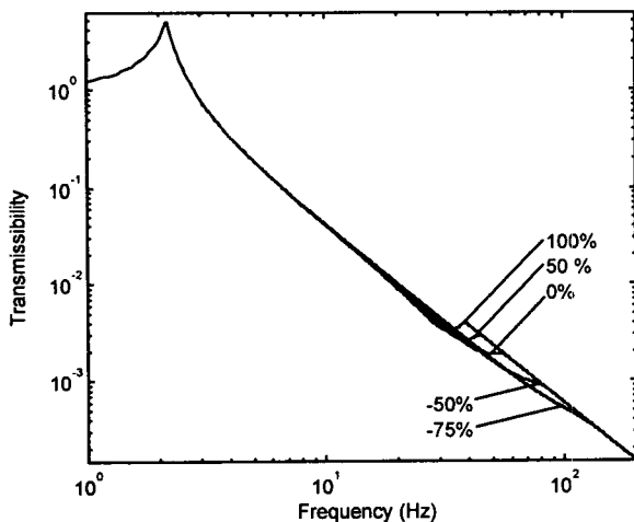
Fig. 11 Effect of inertia track length on MR mount performance
