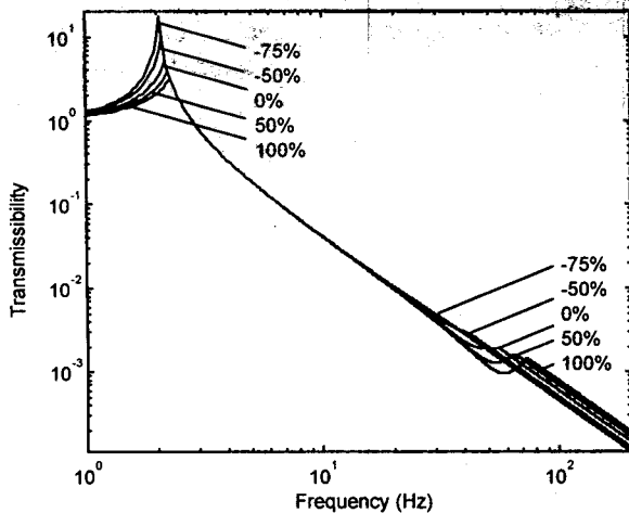
Fig. 14 Effect of volumetric stiffness on MR mount performance
