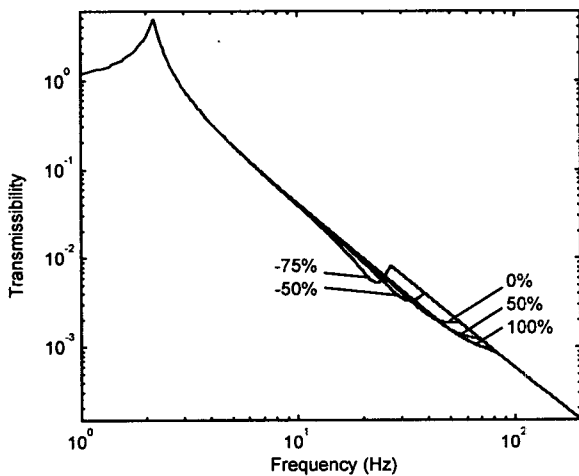
Fig. 10 Effect of inertia track area on MR mount performance
