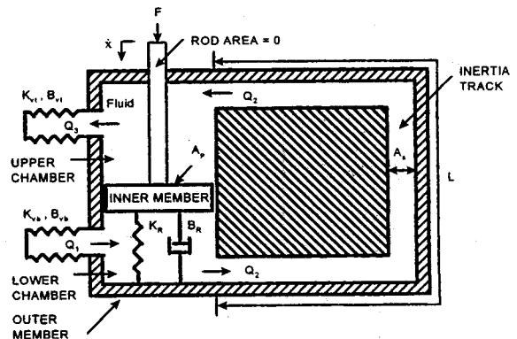
Fig. 3 Mechanical model of a fluid mount
