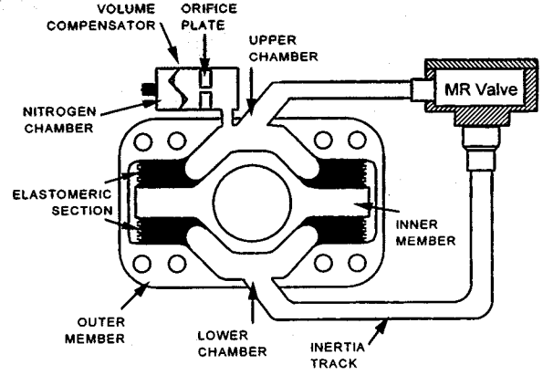
Fig. 2 Schematic diagram of a magneto-rheological mount
