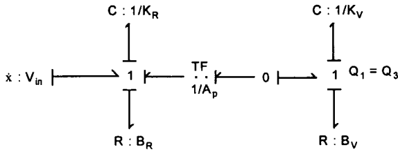
Fig. 6 Bond graph model of the closed-orifice mount
