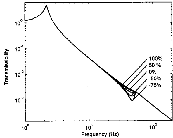
Fig. 12 Effect of fluid resistance on MR mount performance
