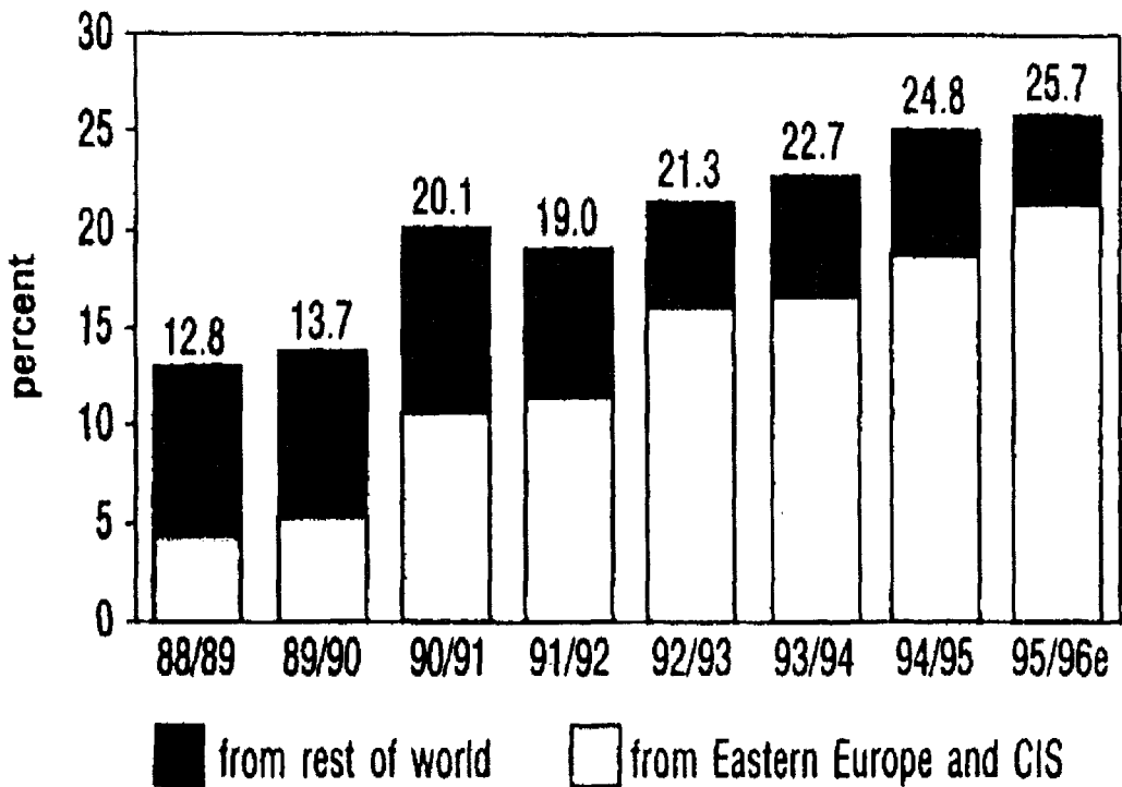
Fig. 1: Fertilizer Imports to EU, In percent of consumption, per fertilizer year (July/June)
