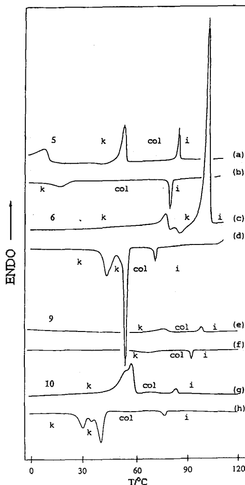
Figure 2. DSC traces (10 °C/min) recorded during the heating scan (a), the cooling scan (b) of 5 , the heating scan (c), the cooling scan (d) of 6 , the heating scan (e), the cooling scan (f) of 9 , the heating scan (g) and the cooling scan (h) of 10 .
