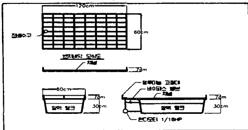
Fig. 1. Schematic diagram of ebb and flow system used in this experiment.
