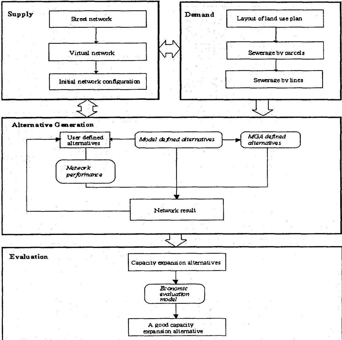
Fig. 4 Sewer Modeling
