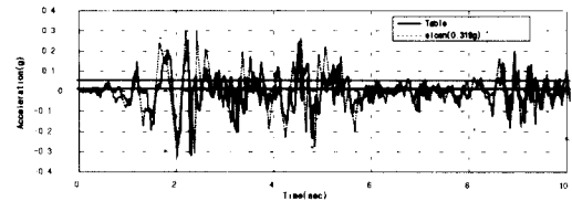
(c) Comparison of the desired and achieved Base motion
