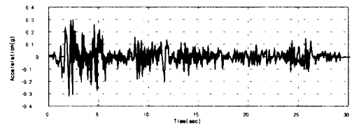
(a) Desired base motion
