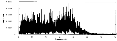
(b) Fourier Transform of shaking table white noise
