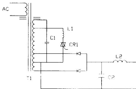
Fig. 3 Single - phase controlled ferro - resonant rectifier circuit.
