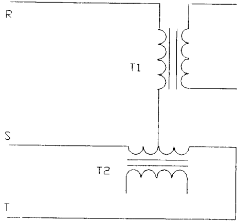
Fig. 4 Three - phase ferro - resonant rectifier ; Scott configuration.
