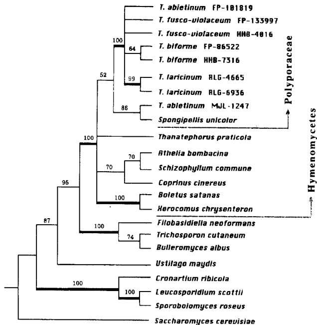
Fig. 1. Phylogenetic tree constructed using parsimony analysis with the heuristic search method of PAUP 3.1.1. It is a bootstrap consensus tree generated from 500 bootstrap replications of 18S rDNA sequences. This tree is identical to the strict consensus tree of 13 equally parsimonious trees requiring 892 nucleotide substitutions, except for the branch for Thanatephorus praticola , which collapsed in bootstrap analysis. The tree has a tree length of 1136 steps, a consistency index of 0.659, and a retention index of 0.650. Bootstrap values are given above branches supported by more than 50% and bold lines are used where branches were significantly supported by more than 90%.
