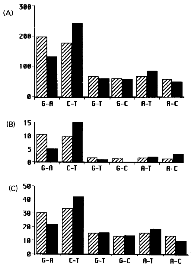
Fig. 4. Distribution of expected and observed base substitution values. (A) all taxa of 18S rDNA sequences. (B) Trichaptum species only of 18S rDNA sequences. (C) Trichaptum species only of ITS1-5.8S-ITS2 sequences. Observed values were inferred from character-state changes of 13 equally parsimonious trees and of the ITS1-5.8S-ITS2 data set. Expected values were calculated by the weighting method of Knight and Mindell (24), which assumes that the probability of a particular type of substitutions is proportional to the frequency of the bases involved. ▨; Expected base substitution values, ■; Observed base substitution value.
