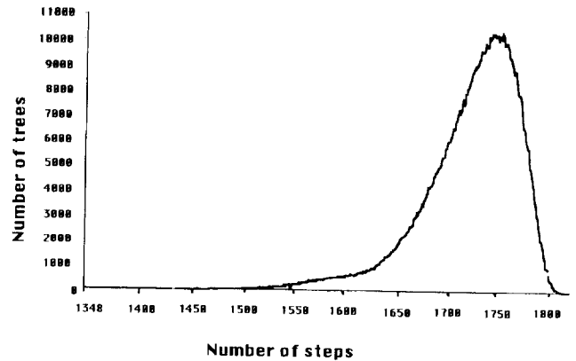
Fig. 2. Tree-length distribution of 1,000,000 random trees generated from possible 5.91 \times 10^{10} rooted trees using the exhaustive and random trees option of PAUP 3.1.1. Tree lengths ranged from a minimum of 1400 to a maximum of 1820. The left skewness measured by the g_1 statistics was -1.33, which was noticeably more skewed than random data whose critical value was -0.09 at P=0.01 .
