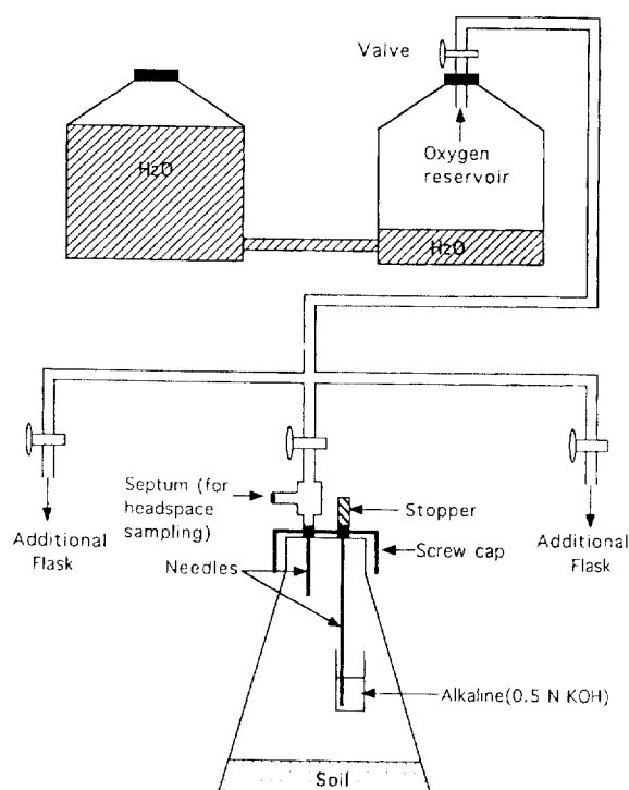
Fig. 1. Sealed aerobic incubation system for BTX compounds in soil.
