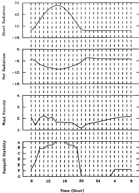
Fig. 9. The diurnal variations of stability categories for urban area.
