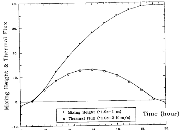
Fig. 6. The diurnal variations of both mixing height and thermal flux.
