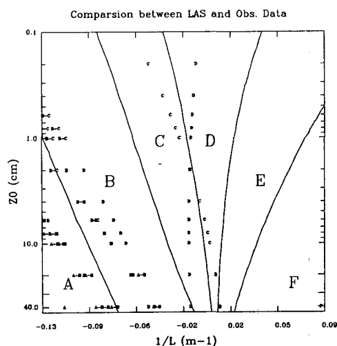
Fig. 8. The comparison of stability categories determined by this model with observational data (Golder, 1972).
