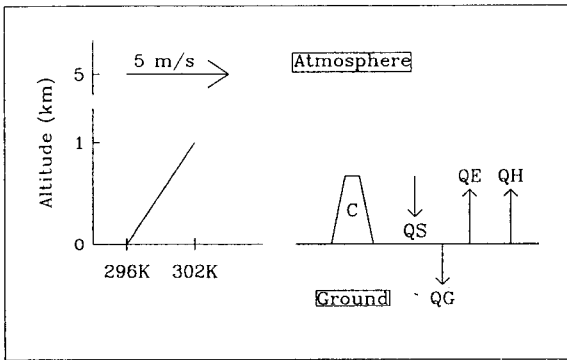
Fig. 1. The schematic diagram of numerical domain.
