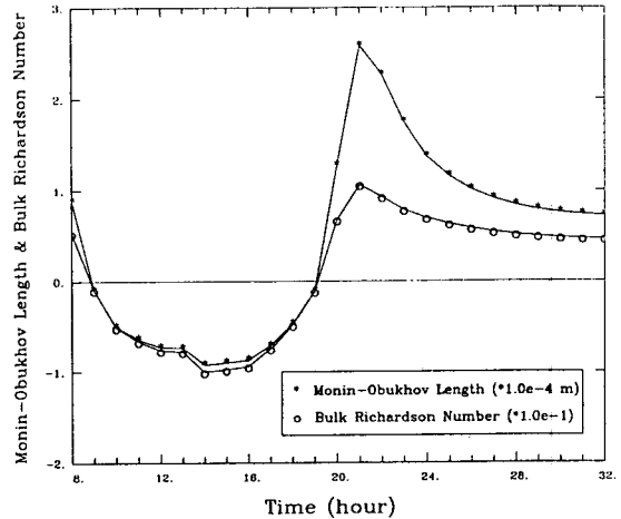
Fig. 5. The diurnal variations of Monin-Obukhov length and bulk Richardson number in the stable surface layer.
