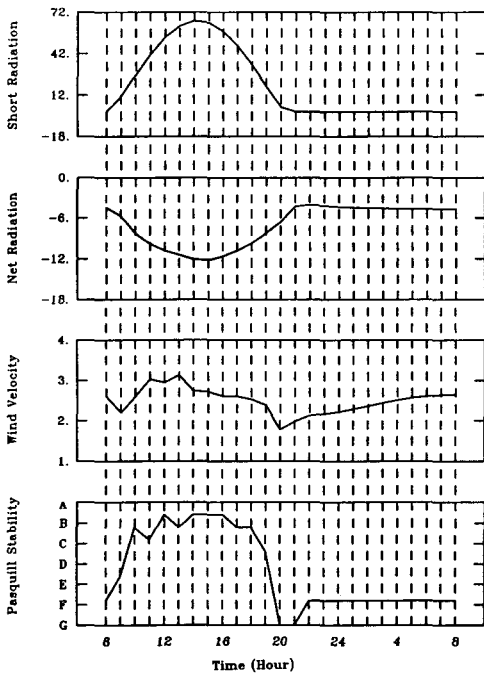
Fig. 11. The diurnal variations of stability categories for rural area.
