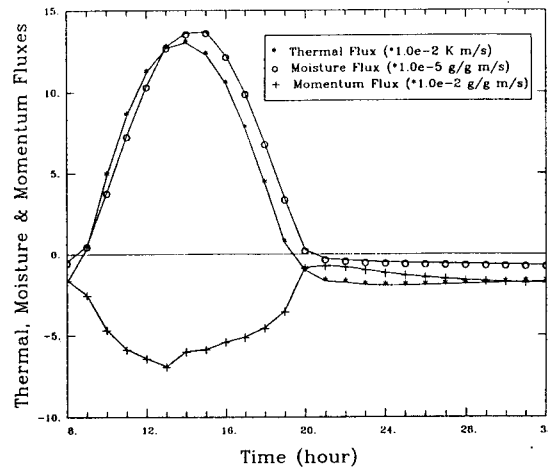
Fig. 3. The diurnal variations of thermal, moisture and momentum fluxes in the surface layer.
