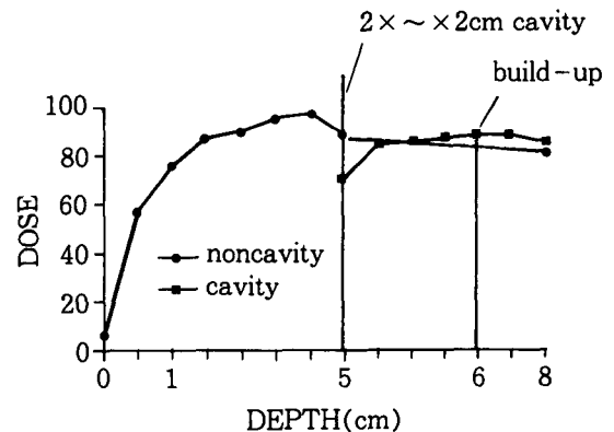
Fig. 4. Depth dose measured in the presence & absence of air cavity(10 MV, FS= 4 \times 4 , 2 \times \sim \times 2 )
