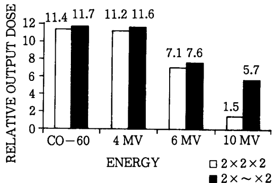
Fig. 12. Relative output measurement after 8 cm in sized materials(FS=6×6)
