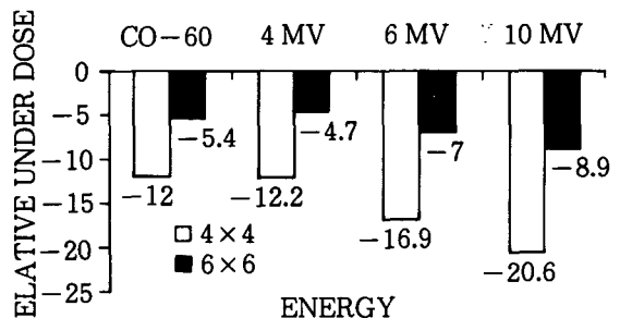
Fig. 8. Relative dose calculation beyond the air cavities(air cavity= 2 \times \sim \times 2 )
