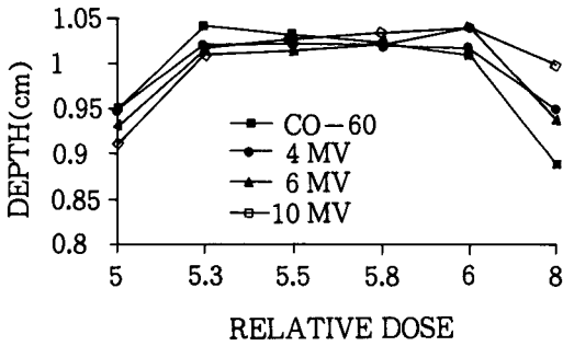
Fig. 9. Relative dose distribution varying to the energy(FS=6×6, air cavity=2×~×2)
