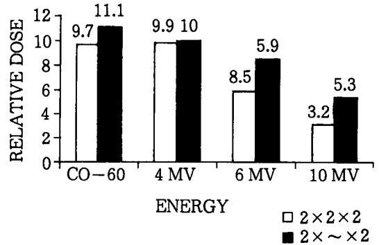
Fig. 11. Relative output measurement after 8 cm sized in materials(FS=4×4)
