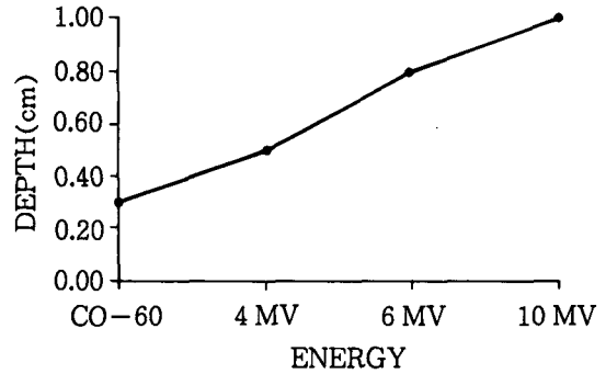
Fig. 2. Rebuild-up point varying to the energy
