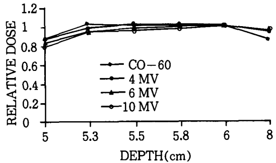
Fig. 5. Relative dose distribution varying to the energy(FS= 4 \times 4 , air cavity= 2 \times \sim \times 2 )
