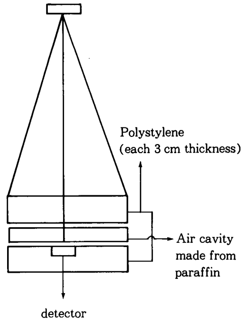
Fig. 1. Irradiation geometry measurements.
