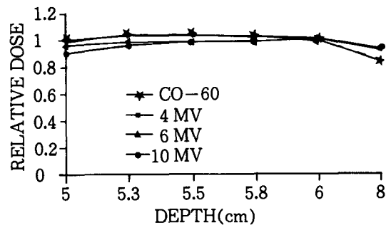
Fig. 6. Relative dose distribution varying to the energy(FS= 4 \times 4 , air cavity= 2 \times 2 \times 2 )
