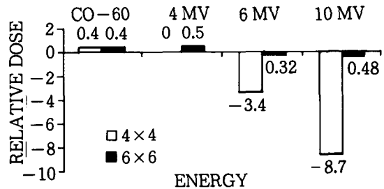
Fig. 7. Relative dose calculation beyond the air cavities(air cavity= 2 \times 2 \times 2 )
