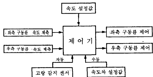
Fig. 1 Schematic diagram of automatic guidance system.
