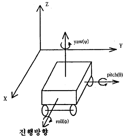
Fig. 3. Coordinate system.
