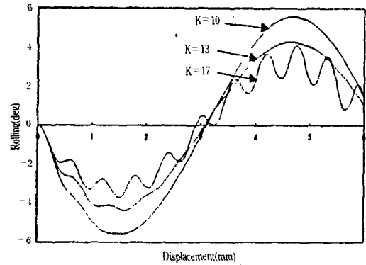
Fig. 8. Altitude control performance of the the PD controller with different values of K_d simulation.
