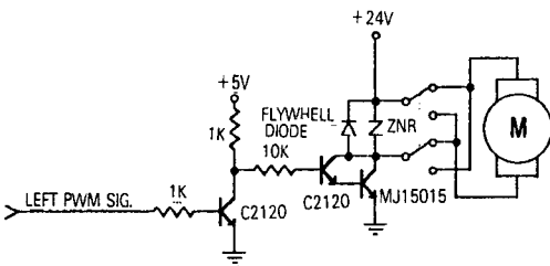
Fig. 4 Circuit diagram of the motor driving unit.
