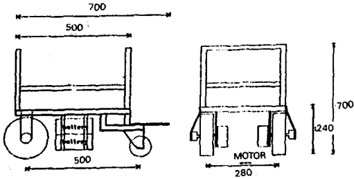
Fig. 6 Shape and dimensions of the cart developed.
