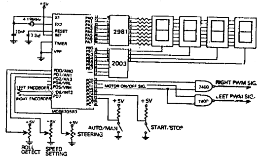
Fig. 5 Circuit diagram of the main controller unit.
