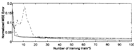
Fig. 3. Learning curves showing the normalized mean square error (NMSE) of networks trained to predict the Mackey-Glass signal an interval t = 6 , into future. The solid curve, point curve, and dash-dot curve are for the ATRN, ATNN and TDNN, respectively.
