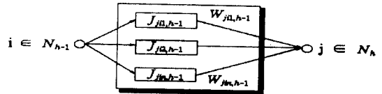
Fig. 2. Delay Box.
