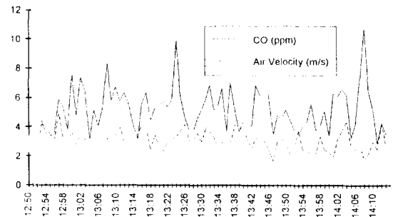
Fig. 3. Temporal variation of CO concentration and air velocity at a fixed location.
