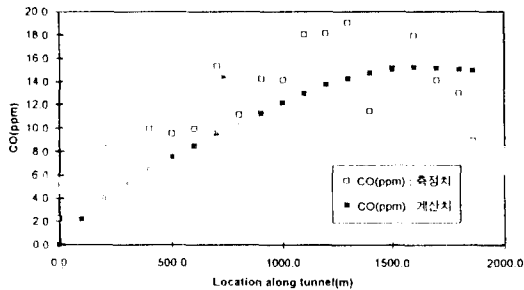
Fig. 2. Comparison of CO concentration along tunnel.
