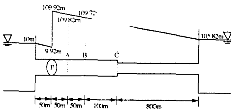
Fig. 3. Initial Condition of Pipe System for Simulation
