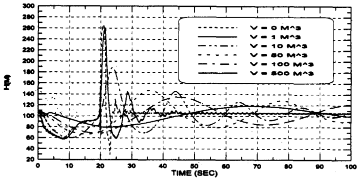
Fig. 4. Attenuation Effect for Different Air Chamber Volumes
