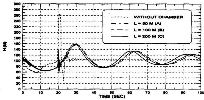
Fig. 5. Attenuation Effect for Different Air Chamber Locations
