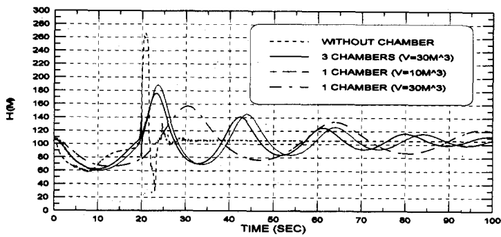
Fig. 6. Attenuation Effect for Separated Chambers
