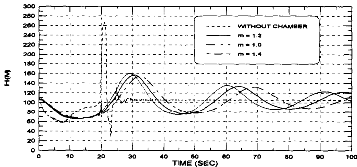
Fig. 9. Attenuation Effect for Different Polytropic Exponents
