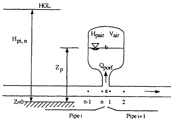
Fig. 2. Pipe System for Simulation
