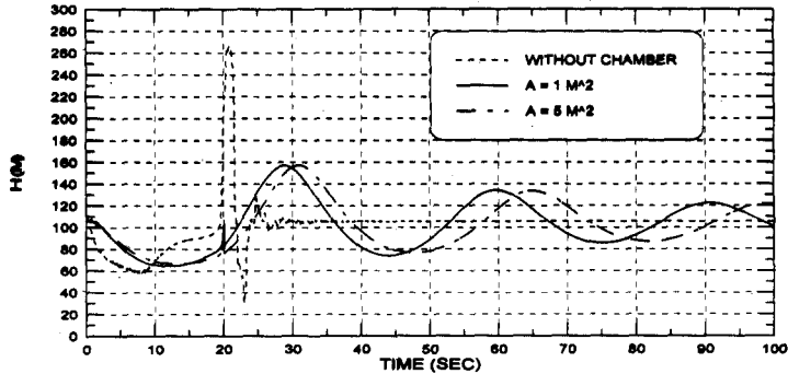
Fig. 7. Attenuation Effect for Different Air Chamber Areas
