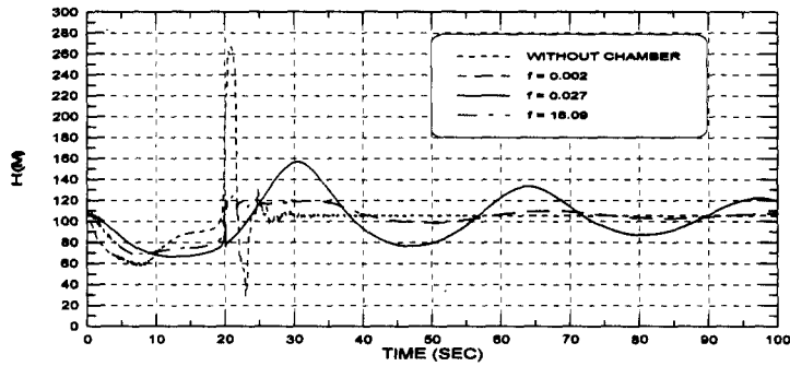
Fig. 8. Attenuation Effect for Different Coefficients of Orifice Loss
