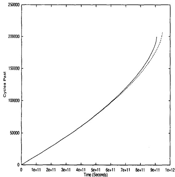
Fig. 1c.— Number of times companion orbits the primary with (solid) or without (dashed) the disk taken into account.
