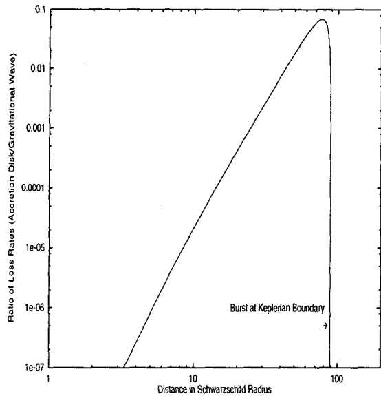
Fig. 1b.— Ratio of the rate of loss of angular momentum due to negative angular momentum accretion and the rate due to gravitational wave emission when the accretion rate is a thousand times the Eddington rate.
