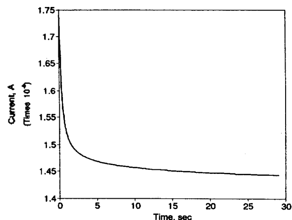
Figure 6. Chronoamperometric curve after background subtraction at the \text{Co(II)(o-BSDT)(H}_2\text{O)}_2 modified carbon ultramicroelectrode for the reduction of 10 mM ferricyanide in 1.0 M \text{KNO}_3 solution. The potential was -0.4 V vs. \text{Hg/Hg}_2\text{SO}_4 .
