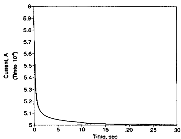
Figure 7. Chronoamperometric curve after background subtraction at the \text{Co(II)(o-BSDT)(H}_2\text{O)}_2 modified carbon ultramicroelectrode for the reduction of oxygen in 1 M KOH solution. The potential was -1.1 V vs. \text{Hg/Hg}_2\text{SO}_4 .
