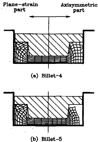
Fig. 8 Grid distortion patterns of final step using Billet-4, Billet-5 in flashless forging
