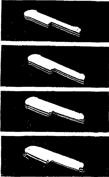
Fig. 12 Material flow patterns of multi-layered plasticine using Billet-2 in forging with flash
