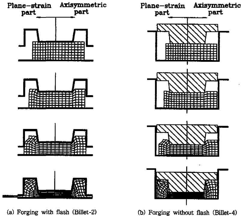
Fig. 11 Die-cavity filling process of grid distortion pattern using Billet-2, Billet-4 in forgings with and without flash
