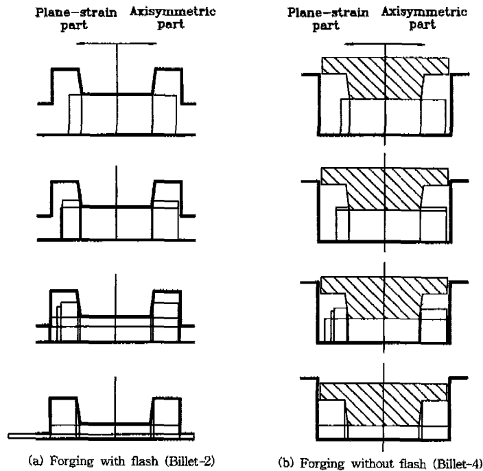
Fig. 10 Die-cavity filling process of element system using Billet-2, Billet-4 in forging with and without flash
