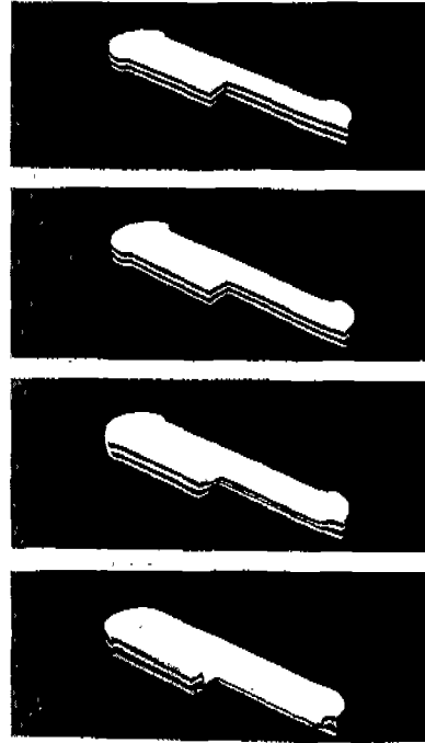
Fig. 13 Material flow patterns of multi-layered plasticine using Billet-4 in flashless forging
