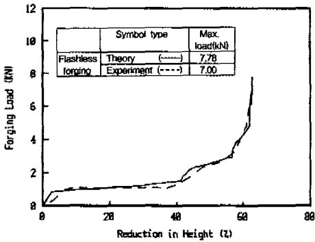
(b) Forging without flash (Billet-4)
