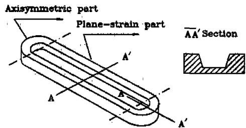
Fig. 1 Analytical model for flashless non-axisymmetric forging
