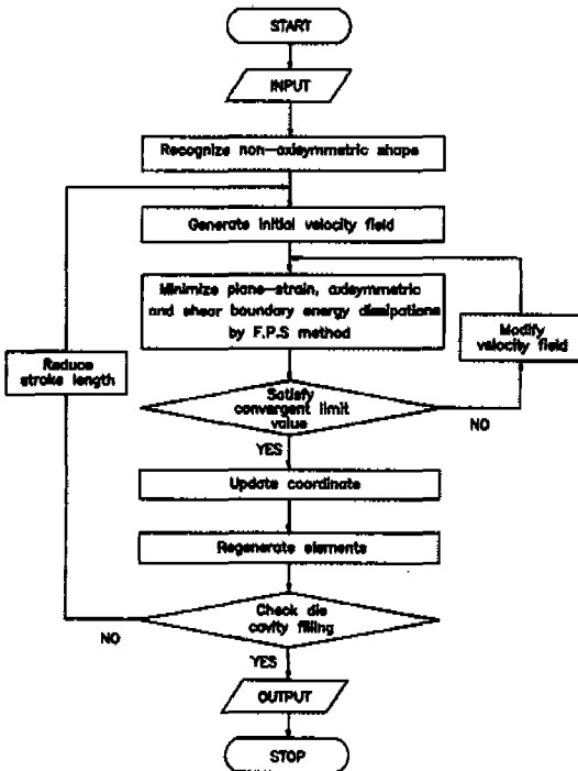
Fig. 3 Flow chart for UBET simulation
