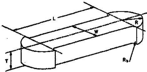
(b) Billet-2 and Billet-4
