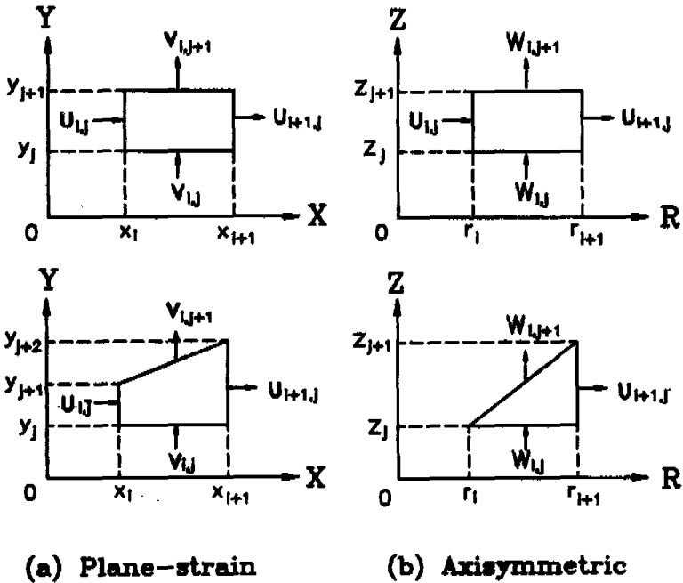
Fig. 2 Normal velocity distribution on the boundaries of elements used in plane-strain and axisymmetric parts
