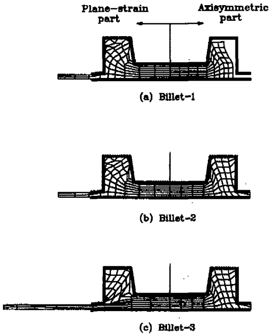
Fig. 6 Grid distortion patterns of final step using Billet-1 Billet-3 in forging with flash
