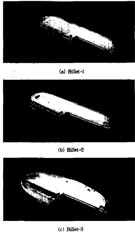
Fig. 7 Flow patterns of final step of multi-layered plasticine using Billet-1 Billet-3 in forging with flash
