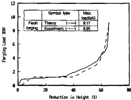
(a) Forging with flash (Billet-2)
