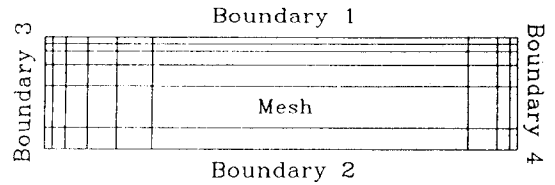
Fig. 2. Macro-mesh of unplapped oil film profiles.
