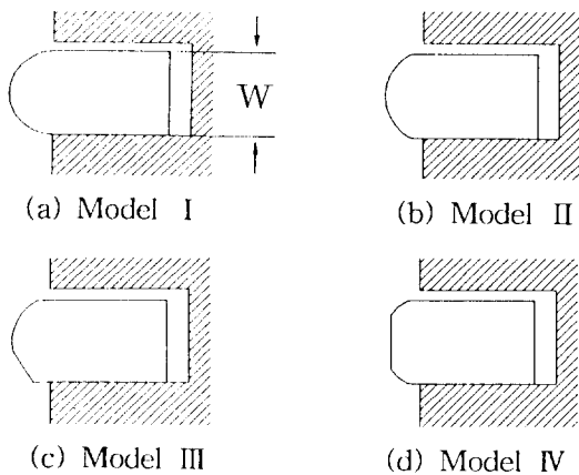
Fig. 1. Models of piston ring profile.
