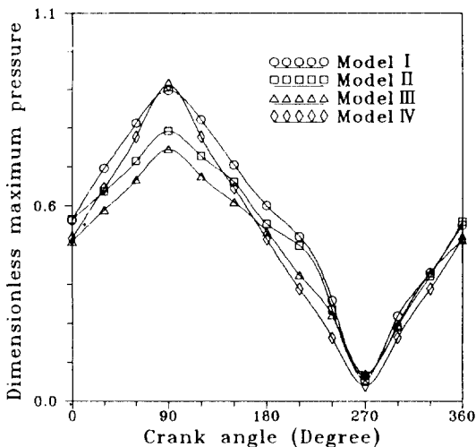
Fig. 4. Dimensionless maximum pressure as a function of crank angle for 1,000 rpm.
