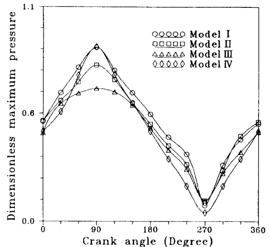
Fig. 6. Dimensionless maximum pressure as a function of crank angle for 2,500 rpm.
