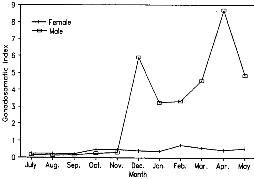
Fig. 5. Monthly changes of the gonadosomatic index in tiger puffer, Takifugu rubripes hatched in 1991 (July 1992~May 1993).
