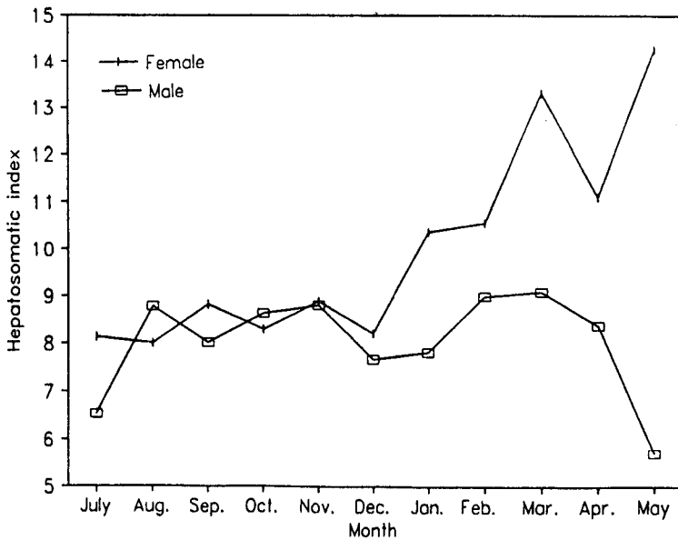
Fig. 6. Monthly changes of the hepatosomatic index in tiger puffer, Takifugu rubripes hatched in 1991 (July 1992~May 1993).
