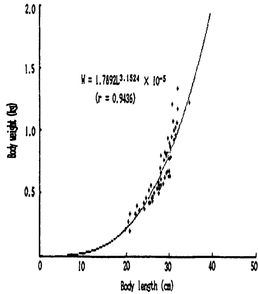
Fig. 2. Relationship between body length and body weight of tiger puffer, Takifugu rubripes hatched in 1991 (July 1992~May 1993).
