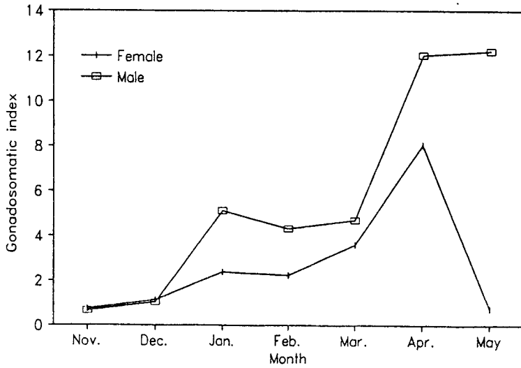
Fig. 7. Monthly changes of the gonadosomatic index in tiger puffer, Takifugu rubripes hatched in 1990 (Nov. 1992~May 1993).
