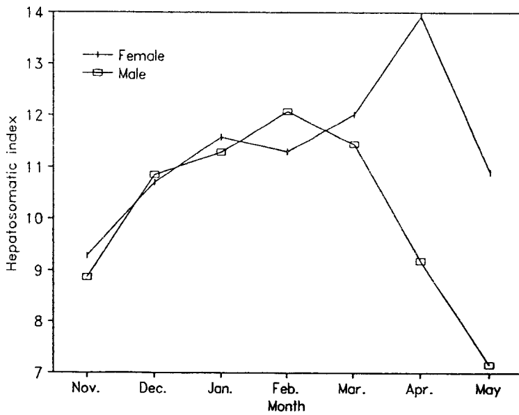
Fig. 8. Monthly changes of the hepatosomatic index in tiger puffer, Takifugu rubripes hatched in 1990 (Nov. 1992~May 1993).
