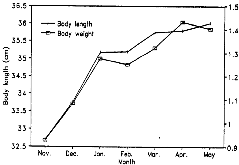
Fig. 3. Variation of mean body length and body weight of tiger puffer, Takifugu rubripes hatched in 1990 by the tank rearing (Nov. 1992~May 1993).
