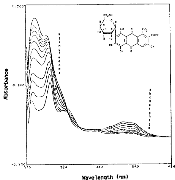
Figure 3. Absorption spectra of carminic acid in various concentrations of \text{Cu}^{2+} . Carminic acid at constant concentration of 1 \times 10^{-5} M was titrated with \text{Cu}^{2+} of varying concentrations; (a) zero M, (b) 2.1 \times 10^{-5} M, (c) 2.9 \times 10^{-5} M, (d) 4.4 \times 10^{-5} M, (e) 5.2 \times 10^{-5} M, (f) 5.7 \times 10^{-5} M, (g) 6.2 \times 10^{-5} M, (h) 6.5 \times 10^{-5} M, (i) 6.8 \times 10^{-5} M, (j) 7.1 \times 10^{-5} M, (k) 7.4 \times 10^{-5} M. Inset shows the structure of carminic acid.
