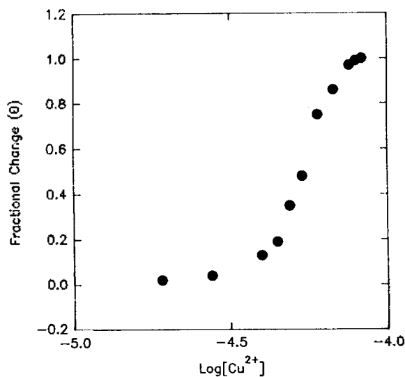
Figure 4. Plot of fractional change ( \theta ) in absorbance at 520 nm vs. \text{Log}[\text{Cu}^{2+}] based on the titration data of Figure 3.
