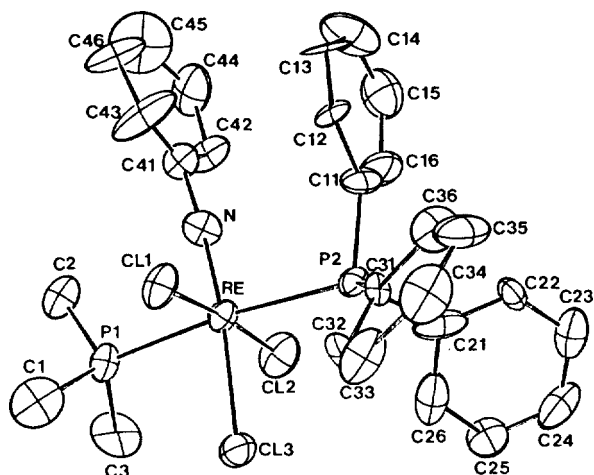
Figure 1. ORTEP drawing of II showing the atom-labeling scheme and 50% probability thermal ellipsoids.
