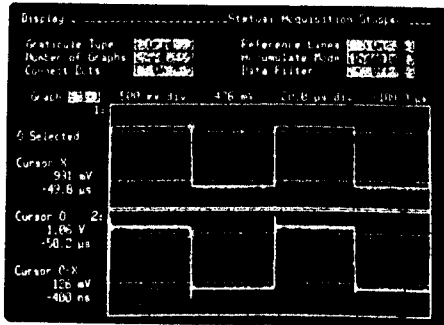
(a) C_1 = 100 [pF]
