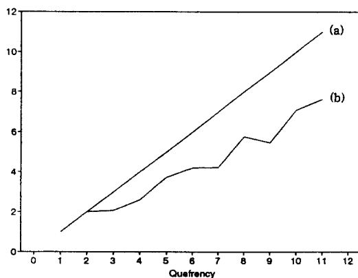
Figure 4 : Weighting factors : (a) quefrency used for d_{\text{QCEP}} , and (b) variance equalizer used for d_{\text{VCEP}} .
