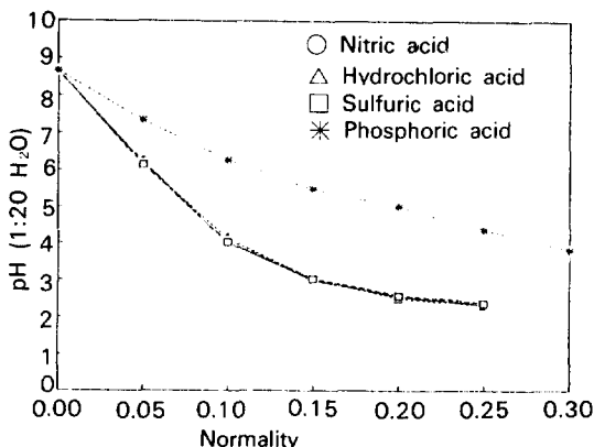
Fig.1 pH curve of carbonized rice hull neutralized by acids
