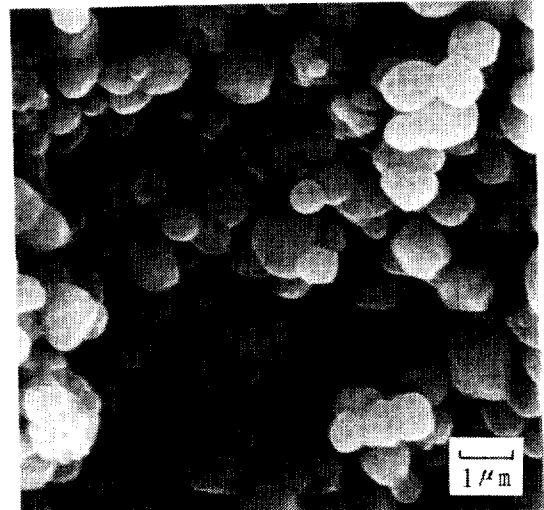
(b) Ca(Ti_{0.99}V_{0.01})O_3
