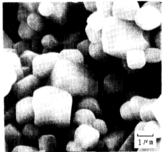
(c) Ca(Ti_{0.98}V_{0.02})O_3
