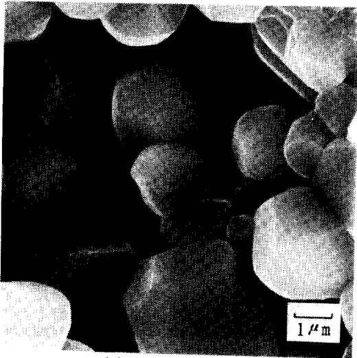
(e) \text{Ca}(\text{Ti}_{0.96}\text{V}_{0.04})\text{O}_3
