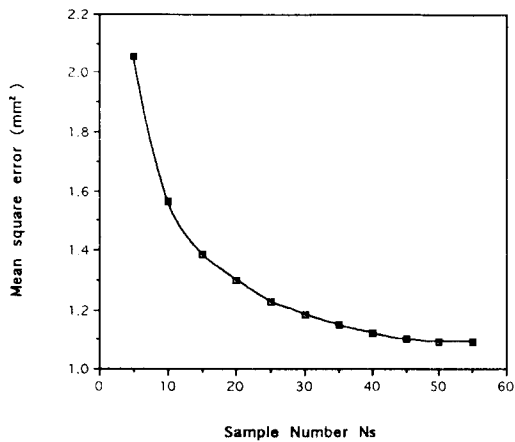
Figure 4. Mean square error decrease with the number of random sampling points
