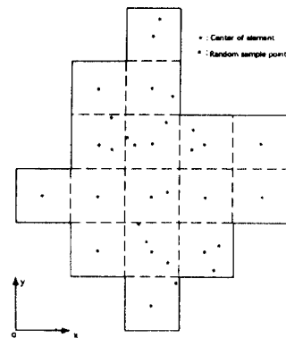
Figure 3. Two ways of selecting representative points : uniform sampling and random sampling
