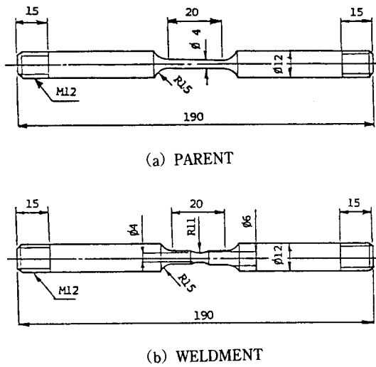
Fig. 1 Specimen geometries
