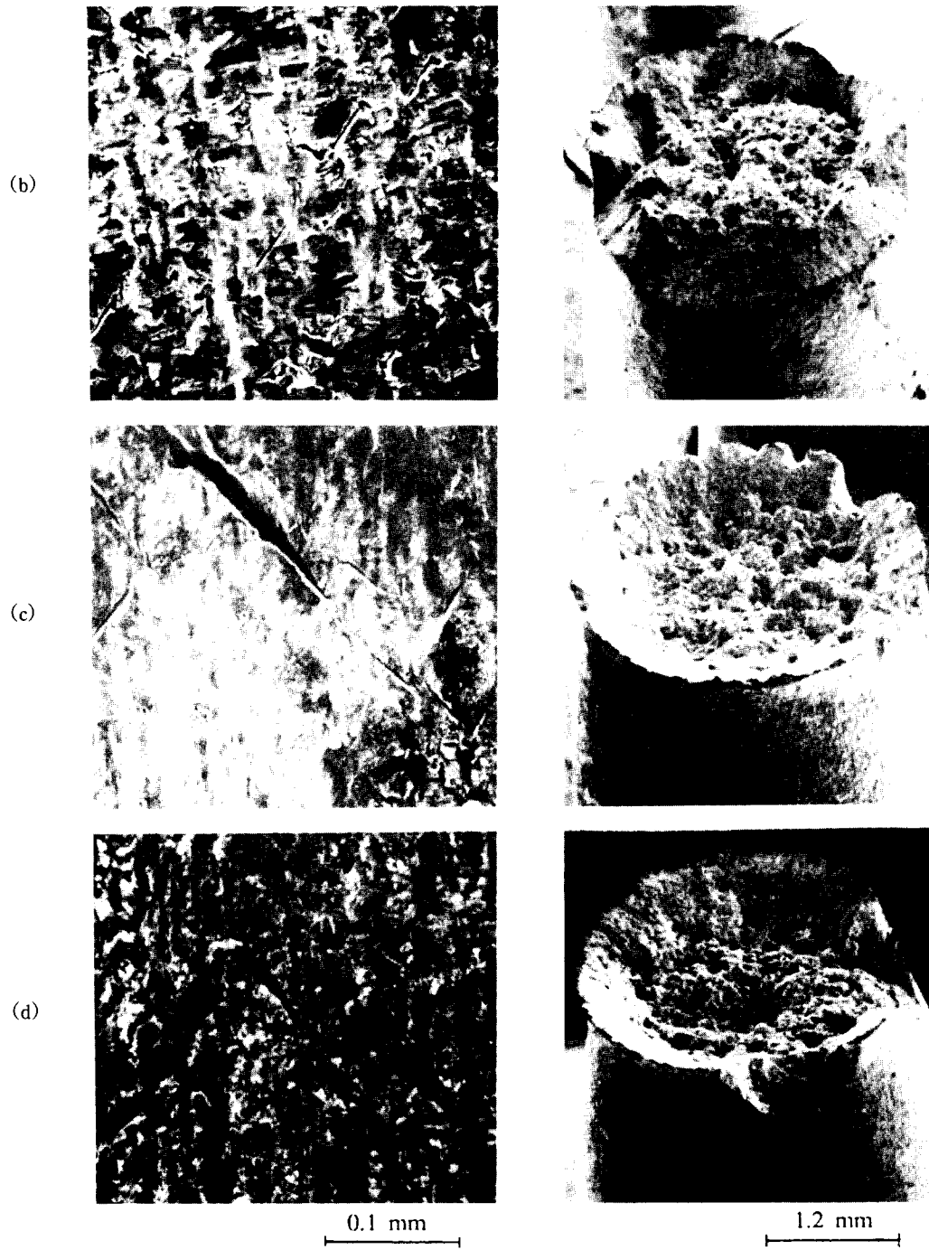
Fig. 9 Micrographs of specimen surface and fracture cross-section of SCM440 after SSRT in s.s.w. (a) strain rate : 1 \times 10^{-5} \text{ sec}^{-1} (c) strain rate : 1.0 \times 10^{-6} \text{ sec}^{-1} (b) strain rate : 4.17 \times 10^{-6} \text{ sec}^{-1} (d) strain rate : 4.17 \times 10^{-7} \text{ sec}^{-1}
