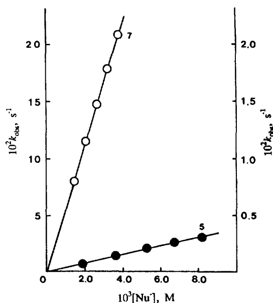
Figure 1. Plots showing dependence of k_{obs} on the nucleophile concentration for the reaction of PNPA with benzohydroxamate (7: left hand side scale) and m -chlorophenoxide (5: right hand side scale) in H 2 O at 25^\circ\text{C} .
