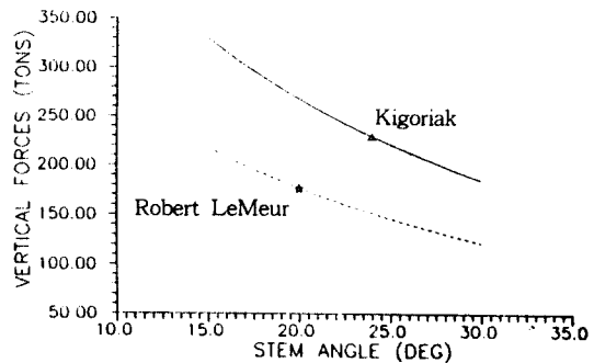
Fig.6 Vertical impact forces against bow stem angles
