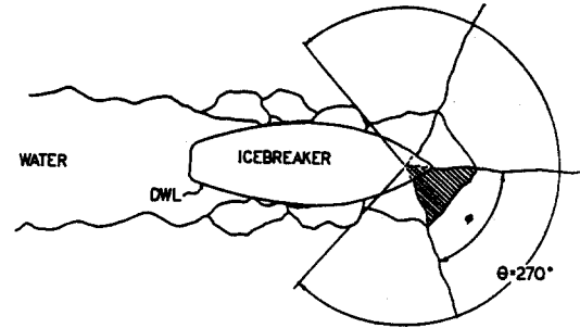
Fig.2 Radial cracks and circumferential cracks in icebreaking process
