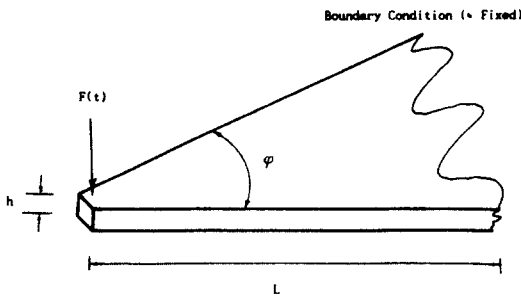
Fig.5 Wedge type model beam for sample calculation
