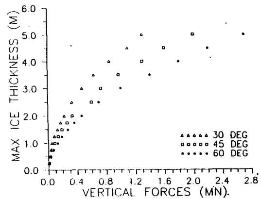
Fig.10 Maximum ice thickness broken versus vertical forces(L=100m)
