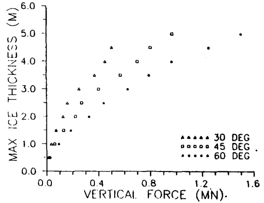
Fig.9 Maximum ice thickness broken versus vertical forces(L=50m)
