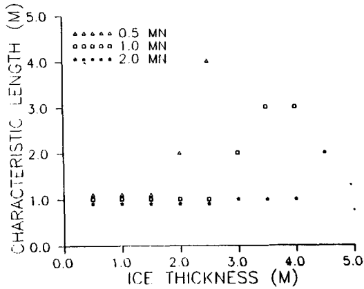
Fig.7 Characteristic length versus ice thickness ( \varphi=60^\circ L=50m)
