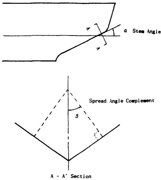
Fig.3 Definition of design parameters in an icebreaker bow
