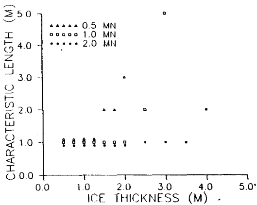
Fig.8 Characteristic length versus ice thickness ( \varphi=60^\circ L=100m)
