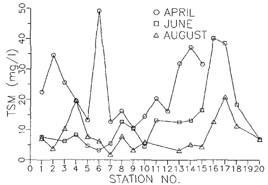
Fig. 8. Concentration of suspended sediment near the bottom.
