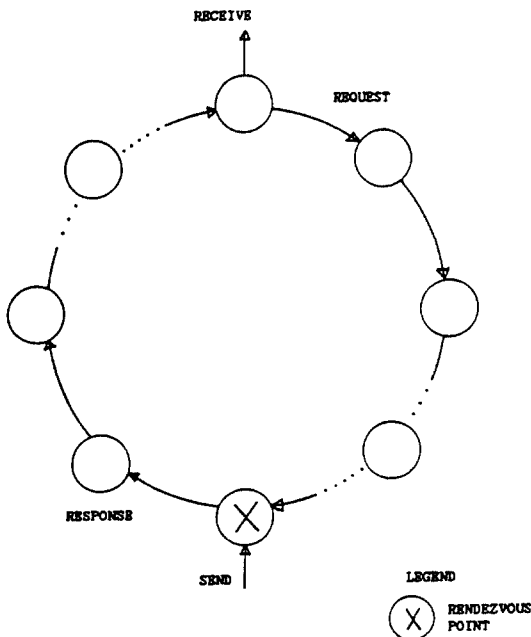
Fig. 1. Transmission Via Rendezvous of Requests and Responses
