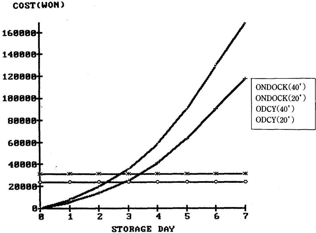
Fig. 3 Cost Comparison according to storage Period
