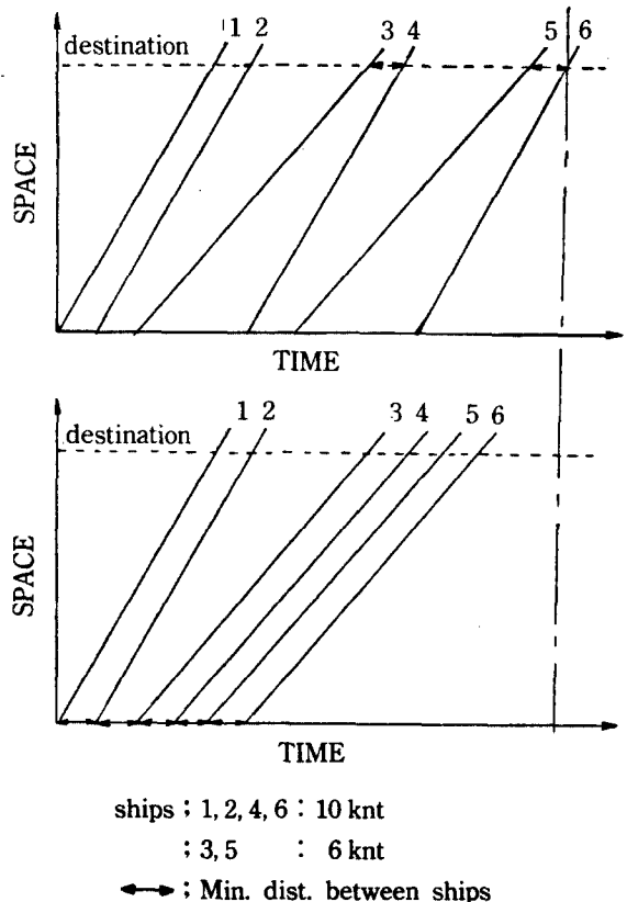
Fig. 3-2 Time-Space diagram
