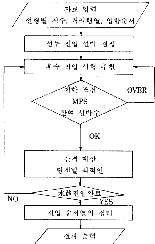
Fig. 3-3 Flow chart of D.P. algorithm for sequencing
