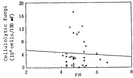
Fig.8. The correlation of cellulolytic fungi with pH.
