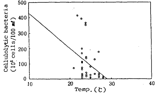
Fig.2. The correlation of cellulolytic bacteria with temperature.
