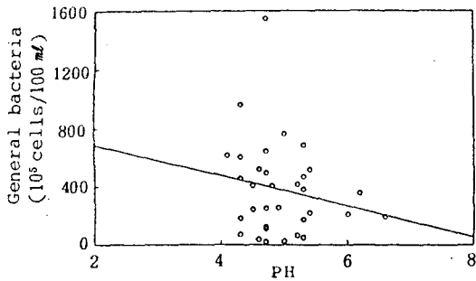
Fig.5. The correlation of general bacteria with pH.
