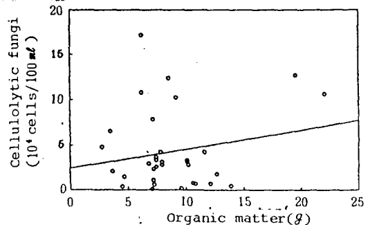
Fig.16. The correlation of cellulolytic fungi with organic matter.
