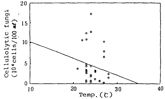
Fig.4. The correlation of cellulolytic fungi with temperature.
