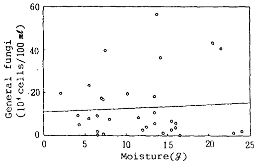
Fig.11. The correlation of general fungi with moisture.
