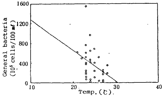
Fig.1. The correlation of general bacteria with temperature.
