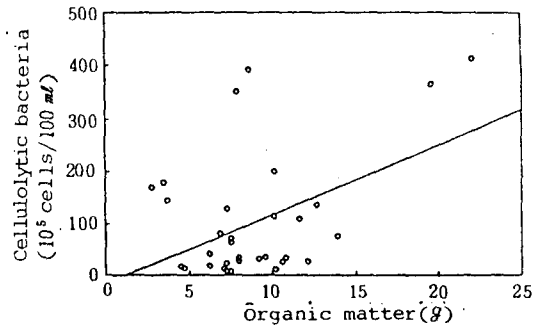
Fig.14. The correlation of cellulolytic bacteria with organic matter.
