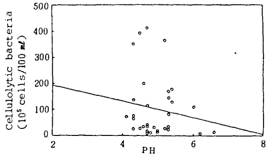
Fig.6. The correlation of cellulolytic bacteria with pH.
