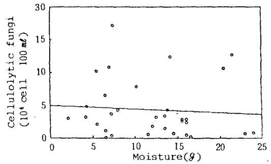
Fig.12. The correlation of cellulolytic fungi with moisture.
