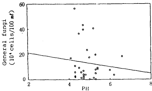
Fig.7. The correlation of general fungi with pH.
