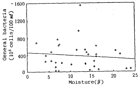
Fig.9. The correlation of general bacteria with moisture.
