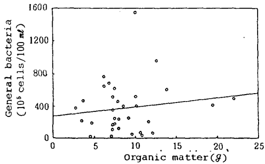
Fig.13. The correlation of general bacteria with organic matter.
