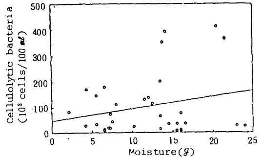
Fig.10. The correlation of cellulolytic bacteria with moisture.
