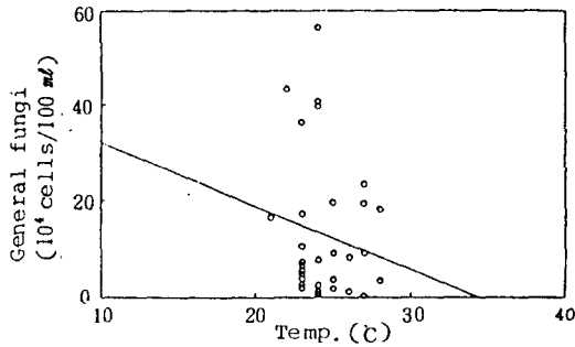
Fig.3. The correlation of general fungi with temperature.
