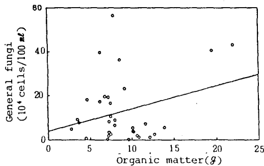
Fig.15. The correlation of general fungi with organic matter.
