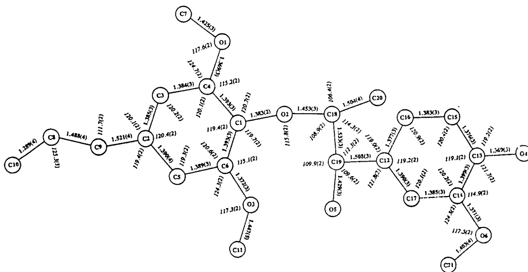
Fig. 2. Bond lengths (Å) and angles ( ^\circ ) of the molecule with their estimated standard deviations in parentheses.
