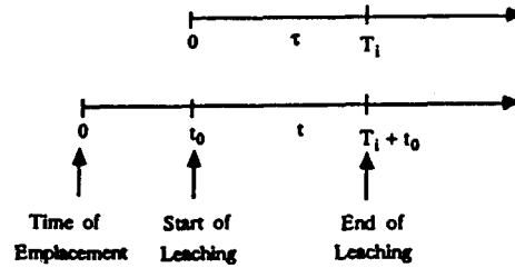
Fig. 4 Comparison of t and \tau
