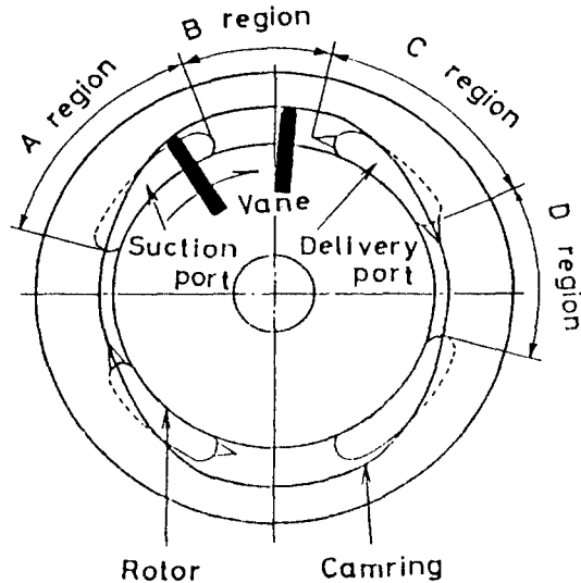
A: Suction port C: Delivery port B: Large arc region D: Small arc region
