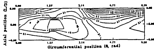
Fig. 11c Temperature Distribution(C), Case #5.
