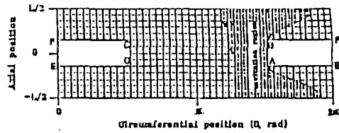
Fig. 11b Calculated cavitation region, case # 5
