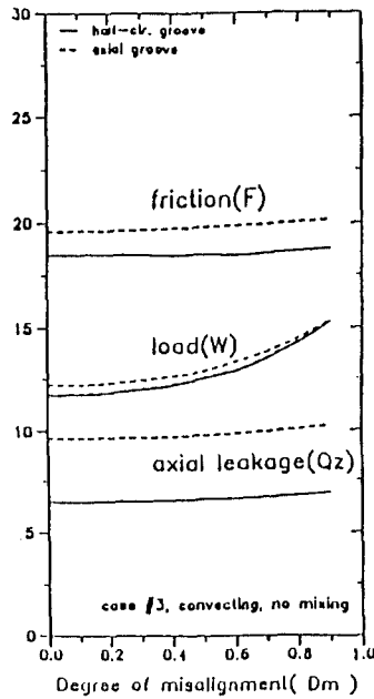
Fig. 10b Convecting, no mixing conditions
