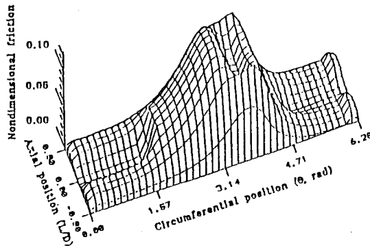
Fig. 7c Non-dimensional friction distribution
