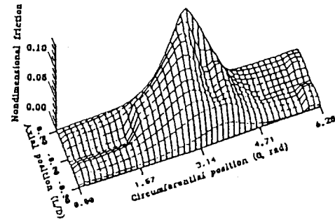
Fig. 11d Non-Dimensional Friction Distribution, Case #5.
