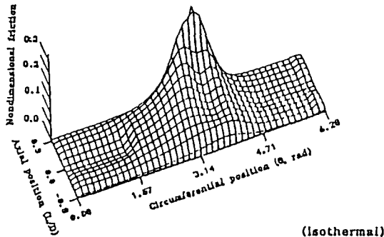
Fig. 11e Non-Dimensional Friction Distribution, Case #1.
