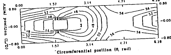
Fig. 8c Temperature distribution (C)
