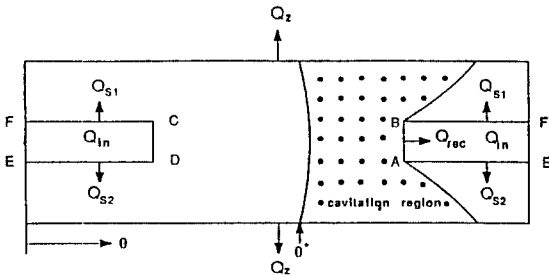
Fig. 4. Digram of Lubricant Flow, with Q_{in} the inlet Oil Flow Rate, Q_{rec} the Recirculating Oil Flow Rate and Q_{s2} , Q_2 the Side Oil Flow Rates. \theta is the Angle of the Beginning of the Cavitation Region. The Groove is in the Rectangle ABFCDEA.
