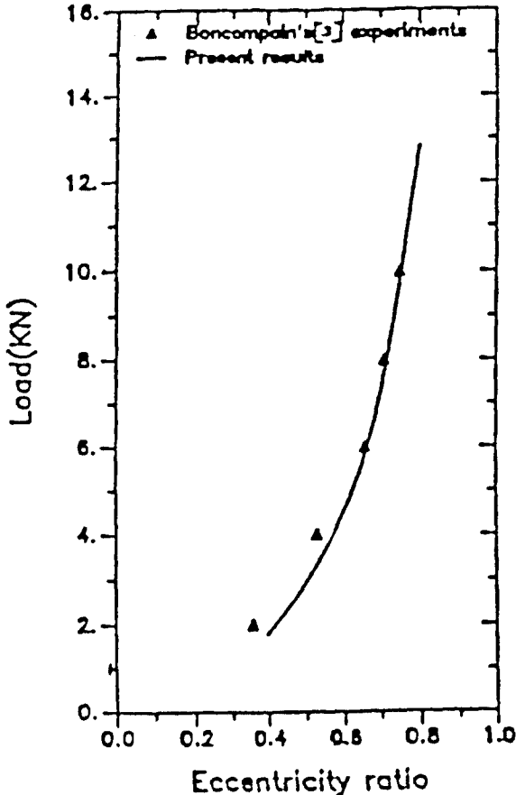
Fig. 6. Comparison of Experimental Results and Computations for the load Capacity Vs. Eccentricity Ratio for and Aligned Bearing with Axial Groove.
