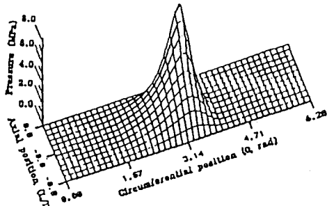
Fig. 11a Pressure Distribution, Case #5, Convecting Walls and Mixing.
