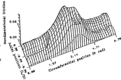
Fig. 8d Non-dimensional friction distribution
