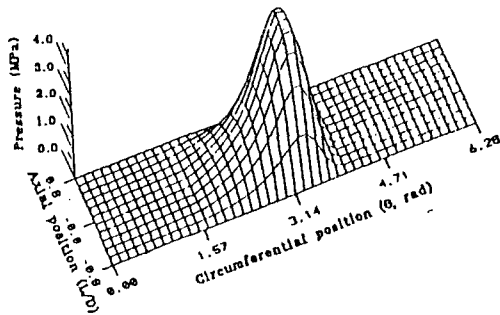
Fig. 8a Pressure distribution
