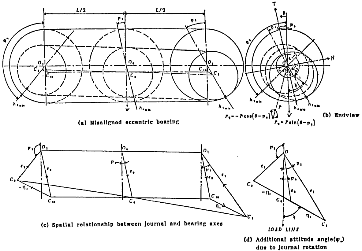
Fig. 3. Attitude of The journal in a Misaligned Bearing C_1-C_2-C_3 the Axis of The Shaft, C_{10}-C_2-C_{20} the Axis of the Shaft if Aligned, and O_1-O_2-O_3 the Bush Axis.
