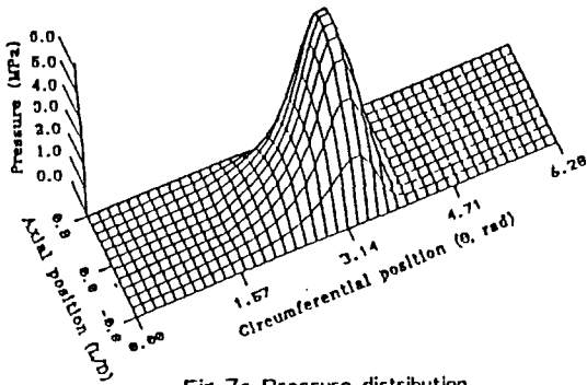
Fig. 7a Pressure distribution
