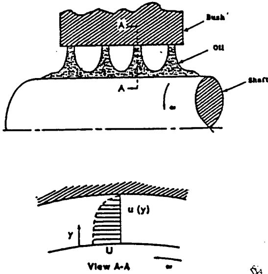
Fig. 1. Oil Streamlets in Cavitated Regions of Journal Bearings[14]
