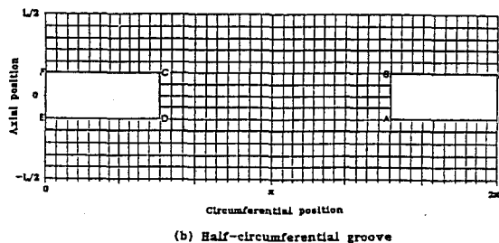
Fig. 5. Location and Size of the Grooves in the Numerical Grid.
