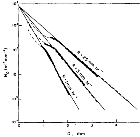
Fig. 3 Measured drop-size distributions (dotted lines) compared with best-fit exponential curves (straight lines) and distributions reported by others (dashed lines). (From Marshall and Plamer, 1948.)
