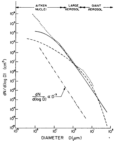
Fig. 1 Number distributions of aerosol obtained from averaging many sets of measurements made in continental air(—), marine air(---), and urban polluted air(···). Also plotted is Eq.(4.1) with \beta=3 but the line is displaced from the other curves for the sake of clarity.
