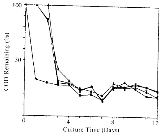
Fig. 5. COD removal efficiencies of four types of activated sludge during dyeing wastewater treatment by semi-continuous cultivation.
