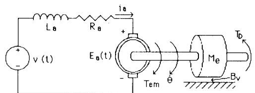
Fig. 1 Integrated system for a motor and its load
