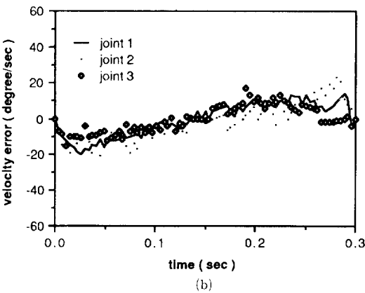
Fig. 5 Trajectory and velocity error curves in each joint with single joint motion. (a) position error, (b) velocity error
