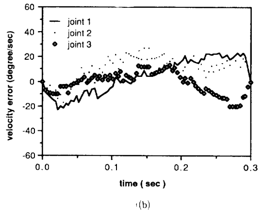
Fig. 6 Trajectory and velocity error curves in each joint with full robot motion. (a) position error, (b) velocity error.
