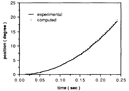
Fig. 4 Position vs. time for a step input for motor 2
