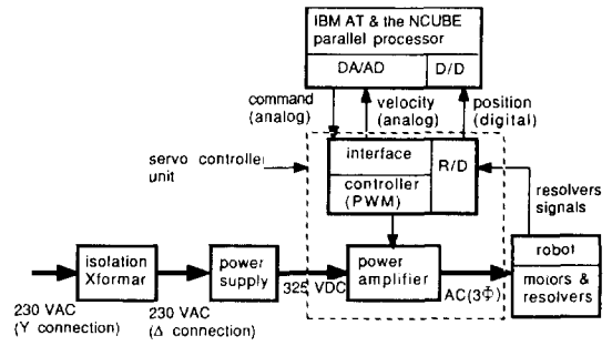
Fig. 3 The Control Hardware for Minnesota Robot
