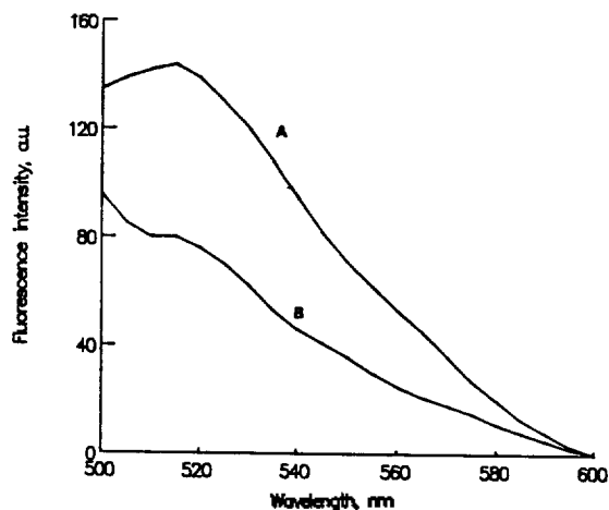
Figure 3. Fluorescence spectra of sample after column separation; A: Baygon (120 ppm) derivative; B: NBD-Cl blank. Spectra were obtained with Farrand MK-1 spectrofluorimeter. Excitation wavelength = 480 nm.
